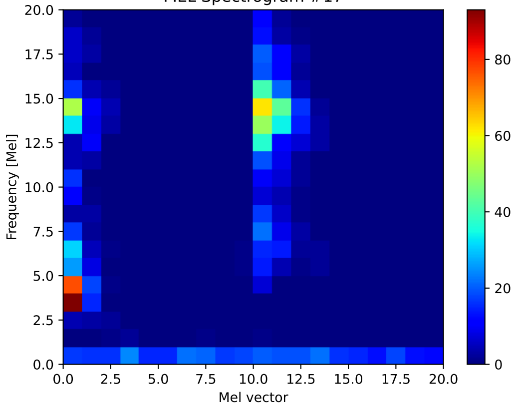
MEL Spectrogram #17
